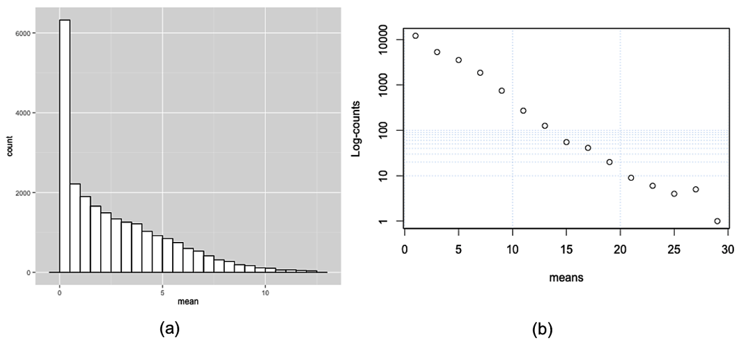
Figure 4. (a) Mean traveled distance distribution. (b) Same distribution plotted over log scale. If the hypothesis of power law holds, (b) should be a straight line.
